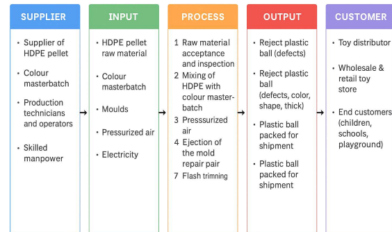
Figure 6 SIPOC Diagram of plastic ball production process
