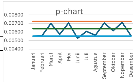
Figure 8. P-chart of monthly defect proportion.
